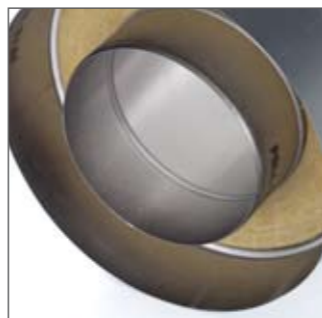
60 mm overlap sikrer en stabil og vandtæt skorsten
